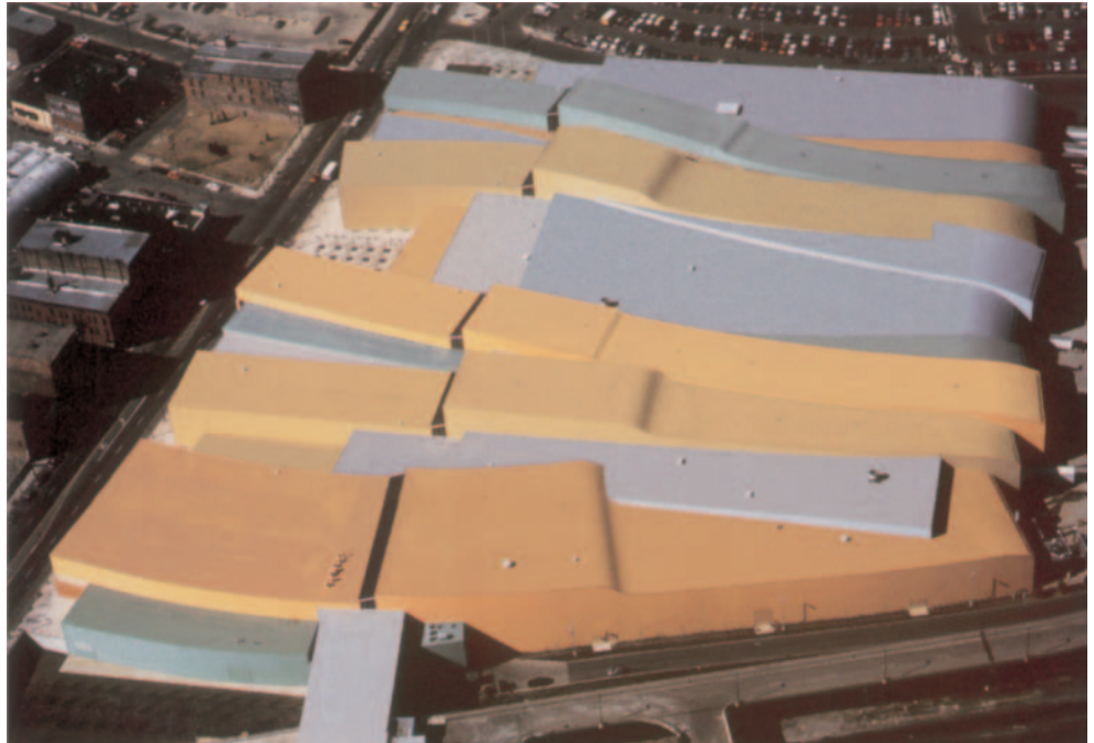
Upper Valley Medical Center, Piqua, Ohio Standing seam metal roof system with kynar color coating.
